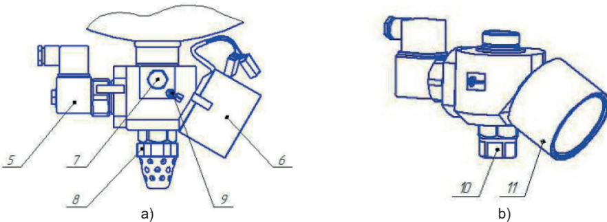
5 - solenoid valve; 6 - electric contact pressure gauge; 7 - safety device; 8 - sprayer; 9 - grounding terminal; 10 - "safety screw"; 11 - protective collar a) a lock and release device with a sprayer; b) a lock and release device with a "safety screw"
