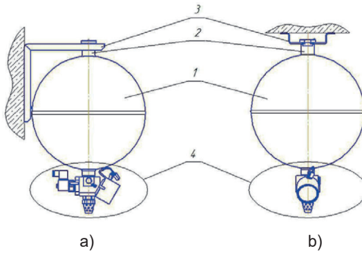
1 - high-pressure container; 2 - pad; 3 - bracket; 4 - lock and release device assembled. a - fixture variant on the wall; b - fixture variant on the ceiling
