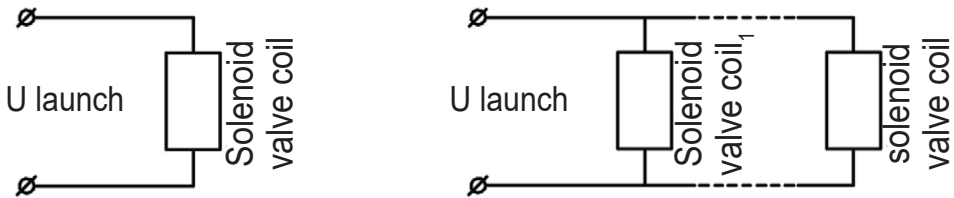
Drawing 6 - EMA connection diagram: a) one unit; b) several units.
