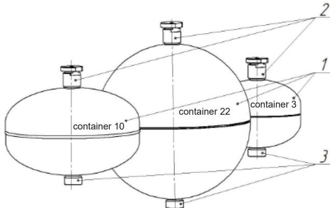
1 - high-pressure container; 2 - pad; 3 - connection Drawing 8 - Container overview
