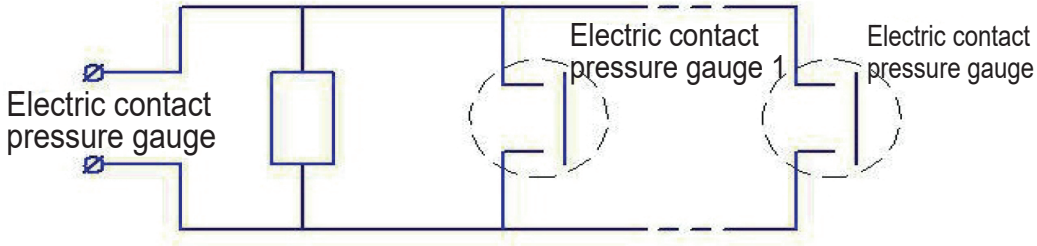
Drawing 5 - Electric contact pressure gauge connection diagram
